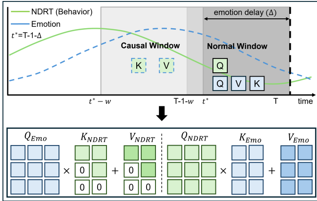
Figure 5: Bidirectional causal cross-attention mechanism. Behavior features (green, NDRT) provide causal context within a past window, while affective features (blue, emotion) query from a delayed window reflecting psychological lag. In parallel, emotion provides global context to behavior, yielding asymmetric but complementary fusion.
