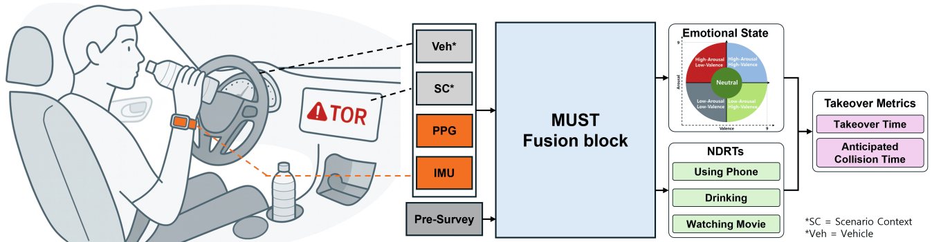
Figure 1: MUST framework integrates multimodal signals and processes them through a fusion block. Extracted features are then analyzed with deep learning models to estimate driver states, non-driving related tasks (NDRTs), and arousal–valence, enabling accurate prediction of takeover-related metrics.
