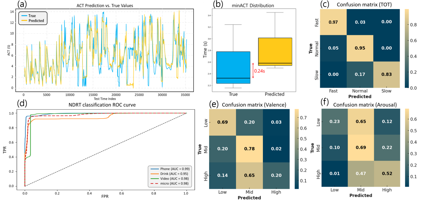
Figure 6: Task-specific performance of the MUST framework. (a) Regression of ACT trajectories against ground truth. (b) Distribution of minACT predictions (box plot). (c) Confusion matrix for TOT classification. (d) ROC curve of NDRT classification. (e) Confusion matrix for valence classification. (f) Confusion matrix for arousal classification.
