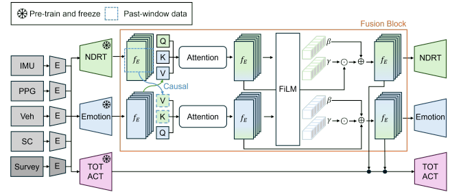
Figure 4: Overview of the MUST fusion architecture. Inputs from multiple modalities are first encoded by task-specific encoders. Within the Fusion Block, we utilize causal cross-attention (Motion \rightarrow Emotion), complementary attention (Emotion \rightarrow Motion), and FiLM integration [66] to produce a fused representation for robust takeover prediction.
