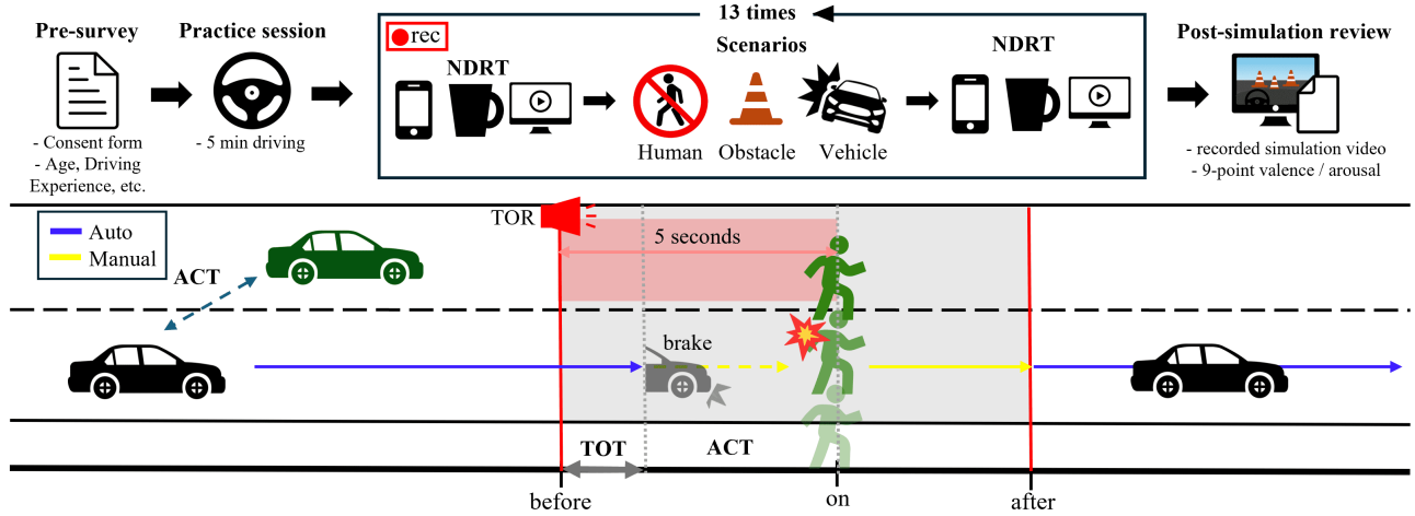
Figure 3: Experimental protocol. Participants completed a pre-survey and practice session before driving 13 takeover scenarios under three NDRTs (smartphone use, drinking, and video watching). TORs were issued in scenarios involving vehicles, pedestrians, or static obstacles, requiring drivers to assume manual control, perform evasive maneuvers, and then return to automation. All sessions were recorded, and post-surveys used the videos for emotion self-report.
