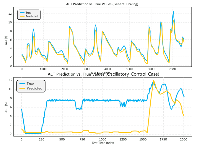
Figure 11: Representative ACT prediction cases. (a) Smooth trajectories across repeated hazard events, where predictions closely track ground truth. (b) Oscillatory control patterns, such as repeated braking or mode-switch toggling, where predictions diverge from actual dynamics.
